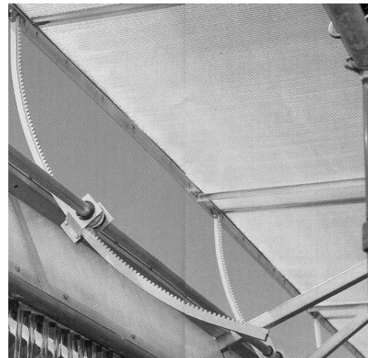
CURVED POWERRACK™ MOUNTED ON GREENHOUSE WITH VENT IN A PARTIALLY OPENED POSITION.
